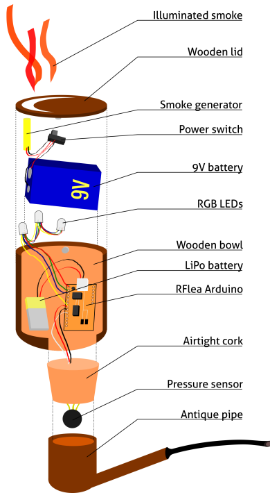
Figure 2: The components used in the Peripipe
